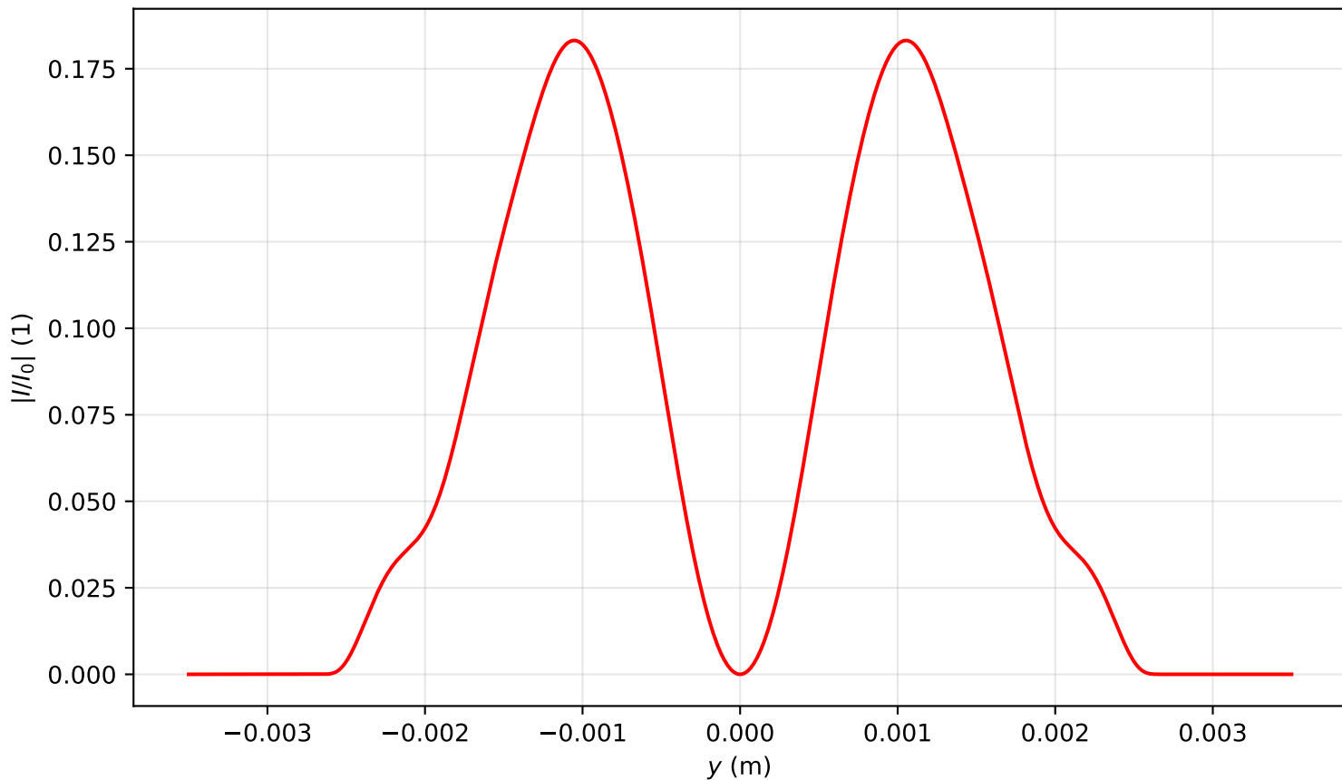
Intensity profile I(x=0, y, z=3.821)/I_0 , P_{in}=0.5P_{cr} , artificial time
